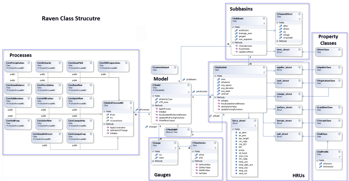
Figure 9.1: RAVEN class diagram
